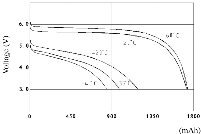
Temperature characteristics(20mA)
