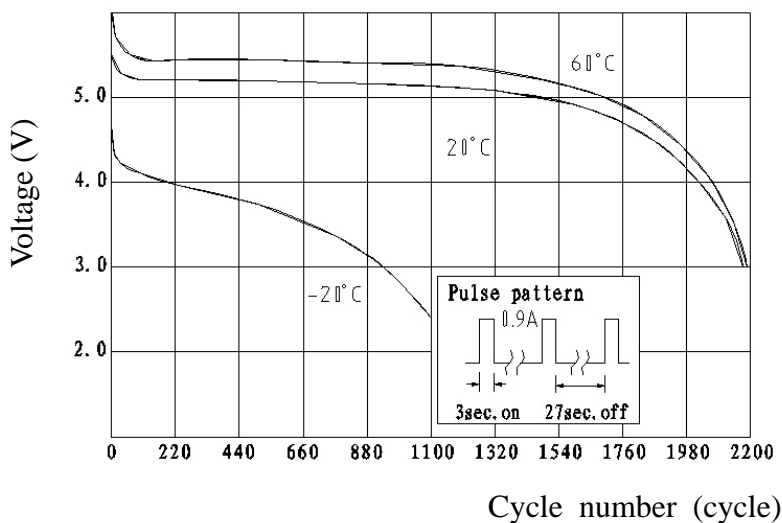
Typical discharge characteristics
