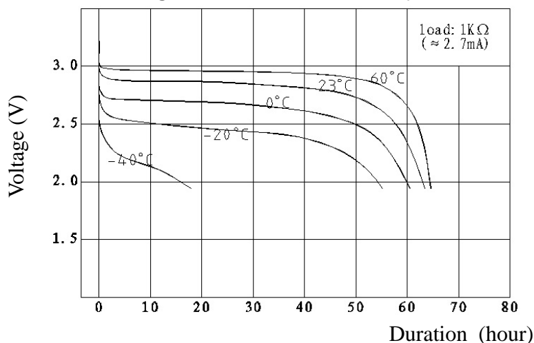
Discharge curve at various temperatures
