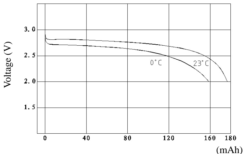
Temperatures characteristics (3mA)
