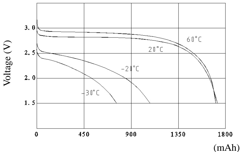
Temperature characteristics(100mAh)
