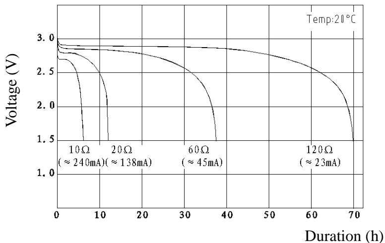
Typical discharge characteristics
