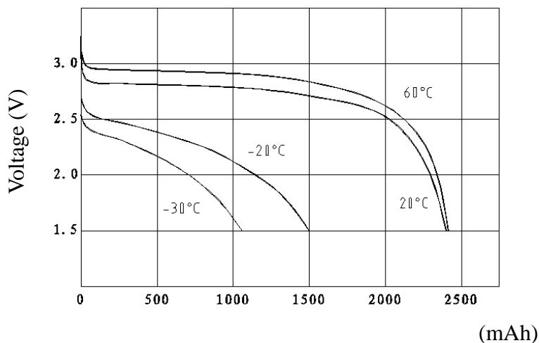
Temperature characteristics(100mAh)
